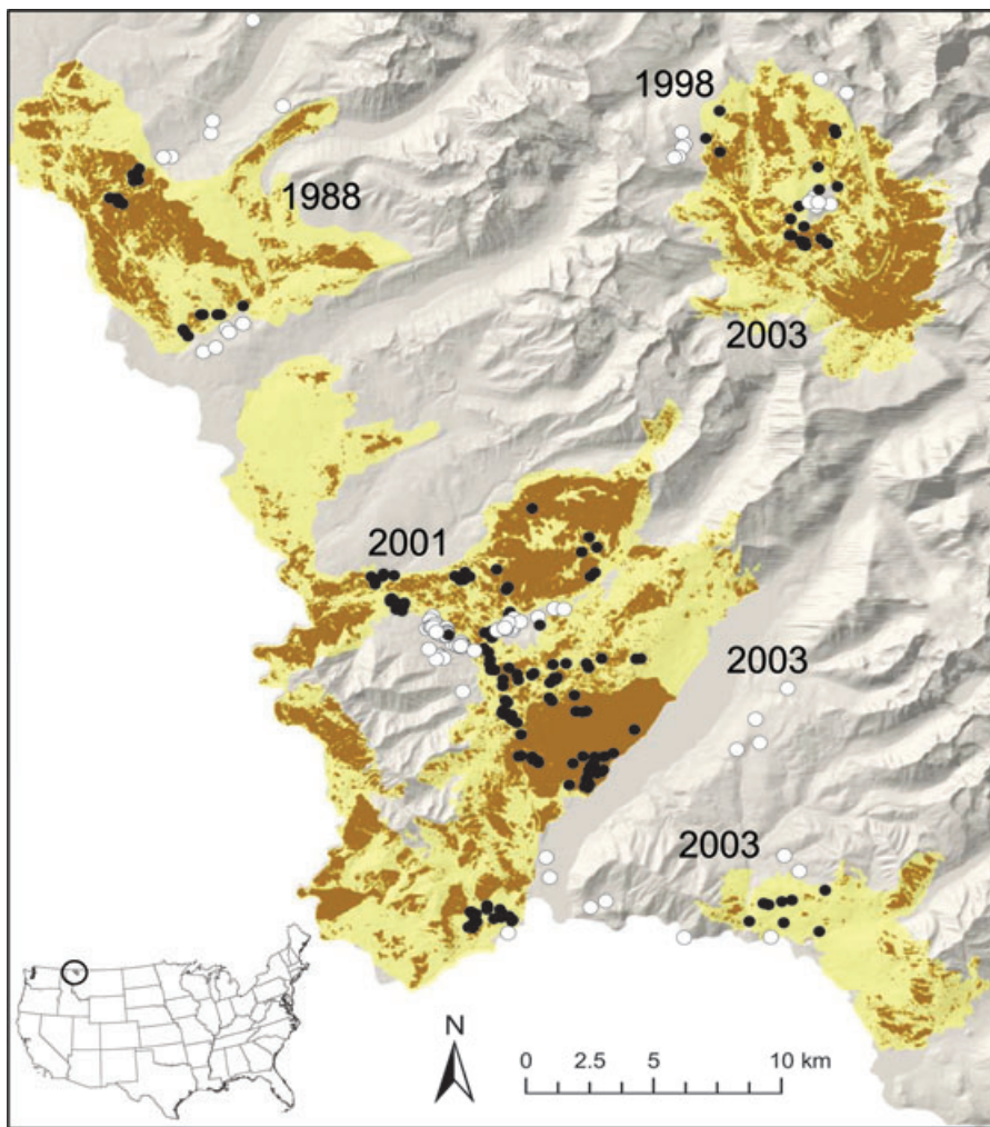
Figure 1. Location of 85 unburned wetlands (white circles) and 183 burned wetlands (black circles) associated with 6 wildfires that occurred in Glacier National Park, Montana (U.S.A.), between 1988 and 2003 (dark brown, severely burned areas; beige, burns of low or moderate severity).
