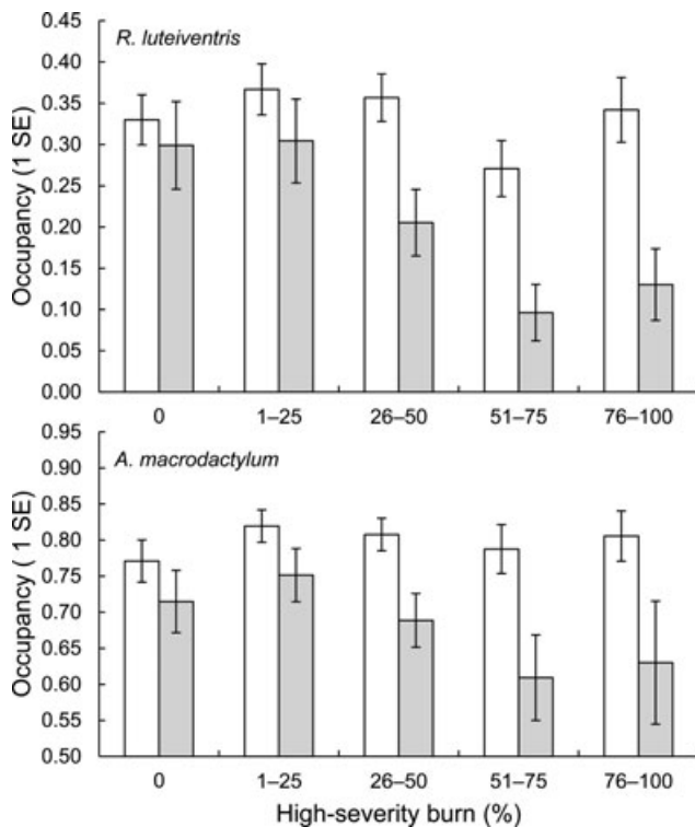
Figure 2. Estimated occupancy (1 SE approximately) of the Columbia spotted frog ( Rana luteiventris ) and long-toed salamander ( Ambystoma macrodactylum ) relative to percentage of area that was severely burned within 500 m of wetlands (x-axis) during the first 6 years after wildfire (unshaded) and years 7–21 (shaded) after wildfire.
