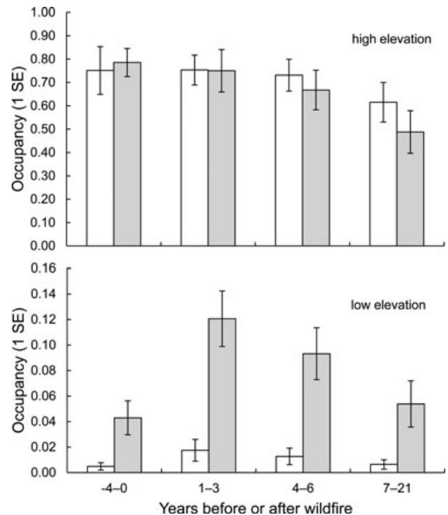
Figure 3. Estimated occupancy (1 SE approximately) of the boreal toad ( Anaxyrus boreas ) in unburned (unshaded) and burned wetlands (shaded) at low elevation (<1465 m) and high elevation (>1866 m) during the 5 summers before wildfire (years –4 to 0) and 1–21 years after wildfire (years 1–3, 4–6, 7–21).
